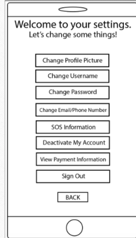
Settings Screen
